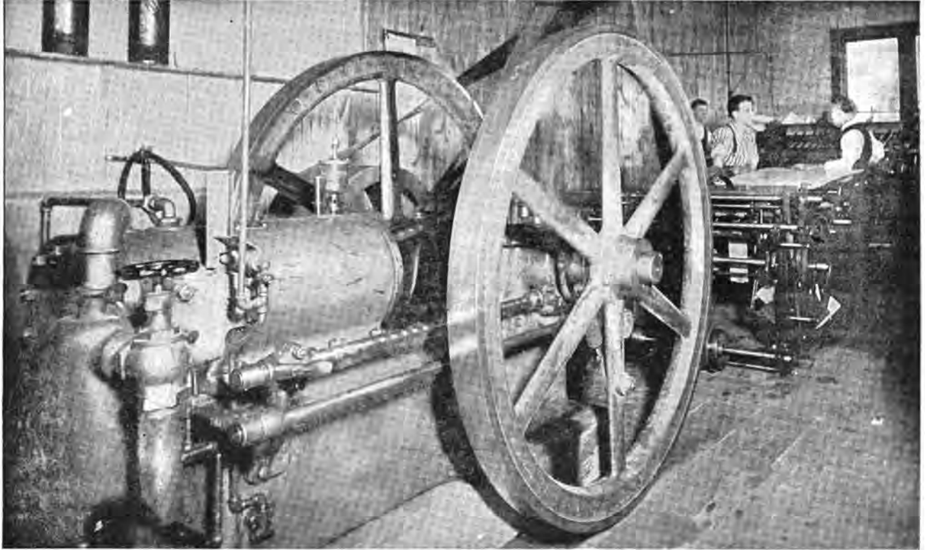
10 H. P. LEWIS GASOLINE ENGINE, WITH DEXTER FOLDER IN THE REAR.
